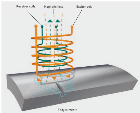
The principle behind eddy current testing
